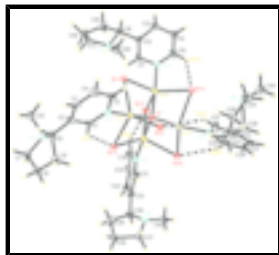
Fig. 1. Molecular structure of the title compound, with atom labels and 30% probability displacement ellipsoids. Intramolecular hydrogen bonds are shown as dashed lines.
